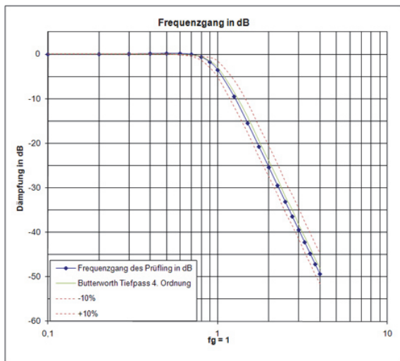
Frequenzgang Butterworth-Filter
