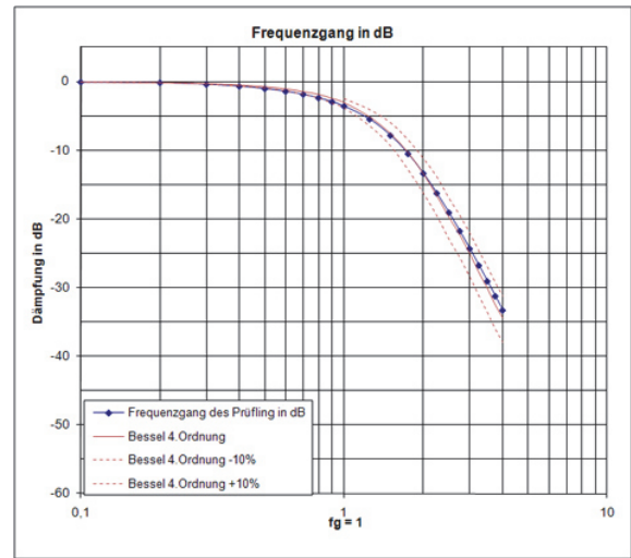
Frequenzgang Bessel-Filter
